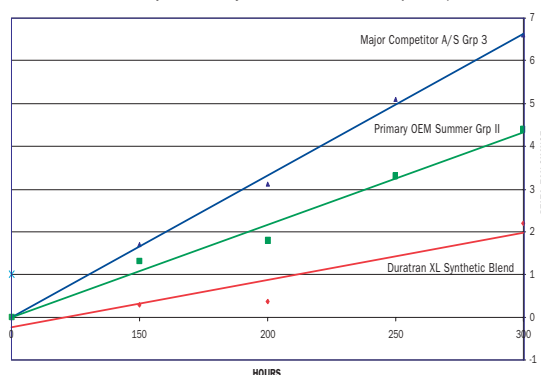
Aluminum Beaker Oxidation Test - ABOT (Delta TAN) Duratran XL Syn Blend vs Major JDM J20C Summer and Competitor A/S
